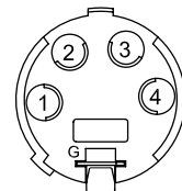
Rear View Male NC4MX-B
