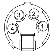
Rear View Female NC4FX
