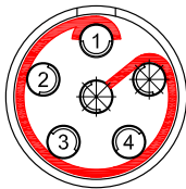
Rear View Lemo
