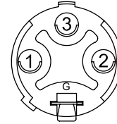
Rear View Male NC3MX
