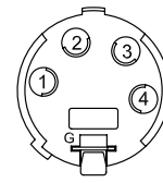
Rear View Neutrik Male NC4MX-B
