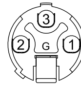
Rear View Female NC3FX
