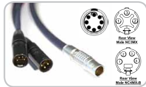
12/24V Split Power Cable
