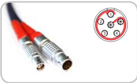
RED Epic 6-Pin to 6-Pin LEMO Power Cable
